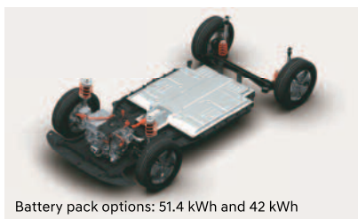
Battery pack options: 51.4 kWh and 42 kWh
